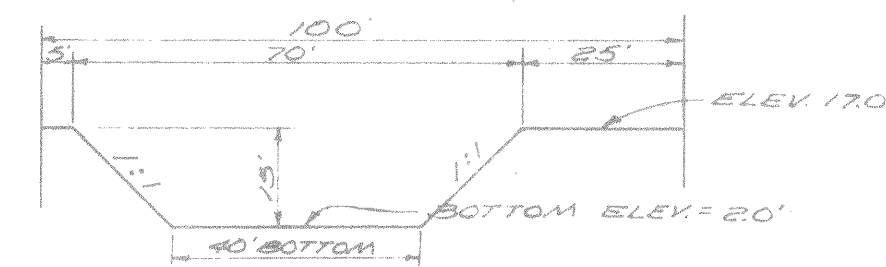
SECTION A-A TYPICAL CANAL CROSS SECTION
